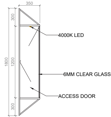
DETAIL 01 SIDE
