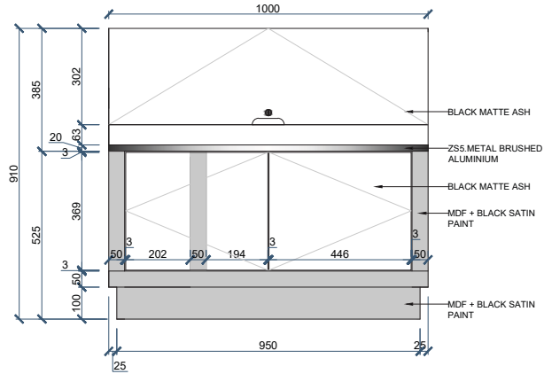
COUNTER REAR VIEW
