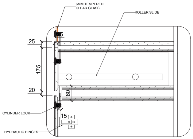
04 SECTION F DETAIL 2 SCALE 1:3
