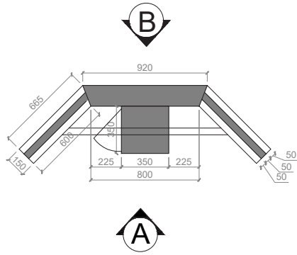
TOP VIEW DISPLAY BACKWALL
