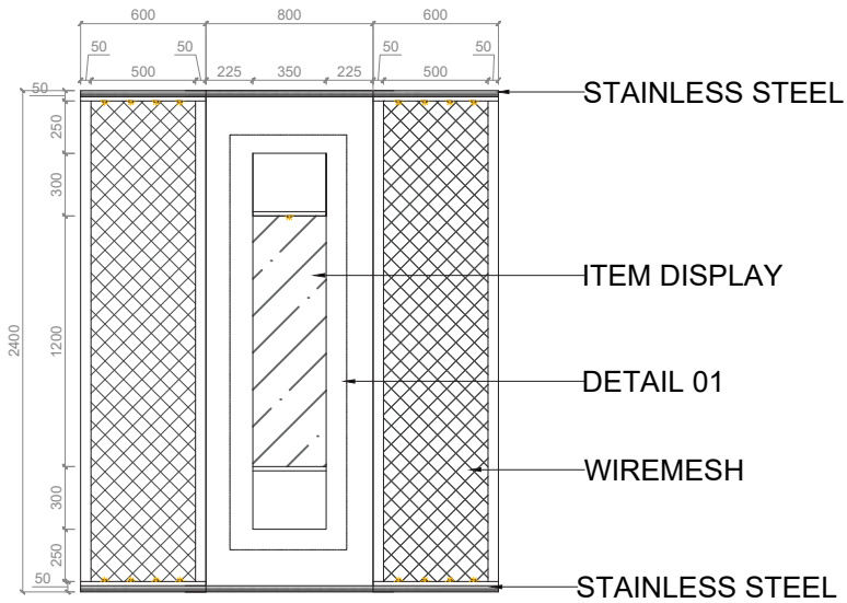
ELEVATION A DISPLAY BACKWALL
